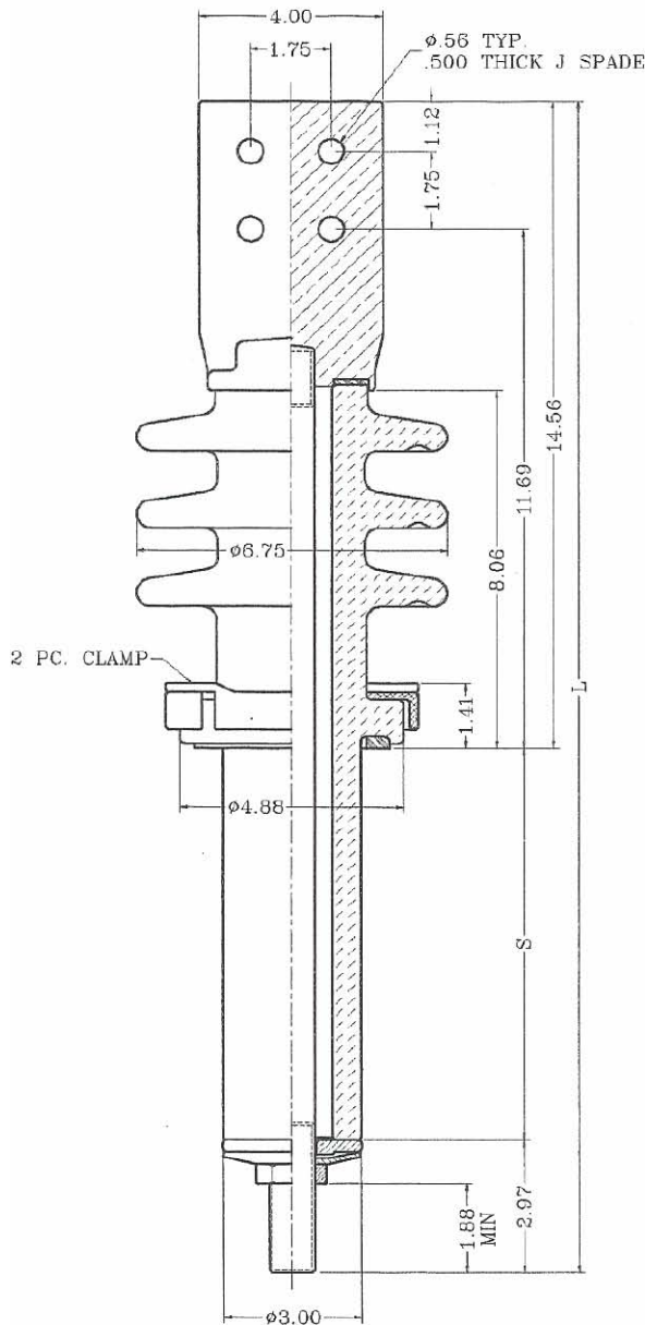
Rev.2, August 1999 2 PIECE EXTERNAL CLAMP
