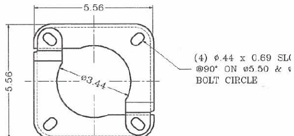
Rev.2, August 1999 2 PIECE EXTERNAL CLAMP
